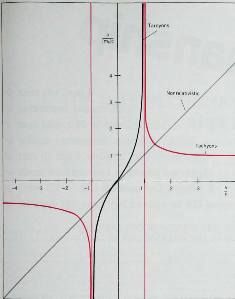
RELATIVISTIC MOMENTUM VS. VELOCITY. The momentum of a tardyon tends to infinity as particle velocity approaches c . Luxons may have any momentum value, but their velocity will always remain at c . As the velocity of a tachyon increases indefinitely, its momentum approaches the limiting value of p = m_*c . —FIG. 4
