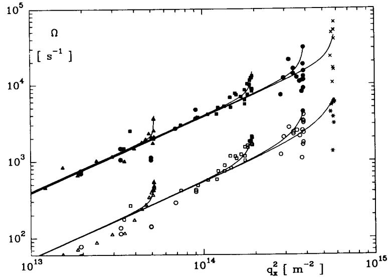
Fig. 10. — Anisotropic dispersion relations of the low and high frequency components of the light scattering signal, displayed as a function of q_{\perp}^2 for various scans at fixed values q of the scattering wave vector modulus \mathbf{q} ; q = 7.2 \times 10^6 \text{ m}^{-1} : open and filled triangles; q = 1.4 \times 10^7 \text{ m}^{-1} : open and filled squares; q = 2.0 \times 10^7 \text{ m}^{-1} : open and filled circles; q = 2.4 \times 10^7 \text{ m}^{-1} : stars and crosses. The lines come from a fit of the complete set of data to the roots of equation (19).
