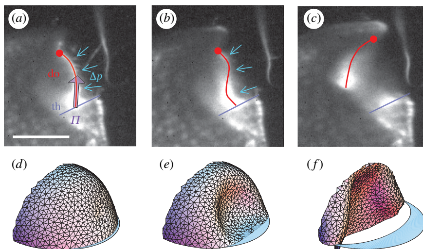
Figure 4. Inversion of trapdoor curvature in U. inflata . (a–c) Buckling of the median door axis, visualized by light sheet fluorescence microscopy. (a) Initially the trapdoor is convex towards the outside of the trap. The force exerted on the door surface owing to water pressure difference \Delta p between the interior of the trap and the outer medium is balanced by the friction force \Pi , exerted by the threshold (th) on the trapdoor (do). (b) Following excitation, the trapdoor becomes gradually concave on its outer side, starting at the trigger hair insertion point. The free edge of the trapdoor is pulled away from the threshold contact area by water pressure. (c) Consequently, the door opens wide. (d)–(f) Dynamic simulation of the trapdoor. Parts (d) and (e) correspond to (a) and (b), respectively, while (f) shows the door only half-way from complete inversion. The scale bar is 500 \mu\text{m} .
